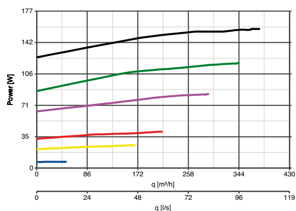
VORT PROMETEO PLUS HR 400 CURVE ASSORBIMENTI
