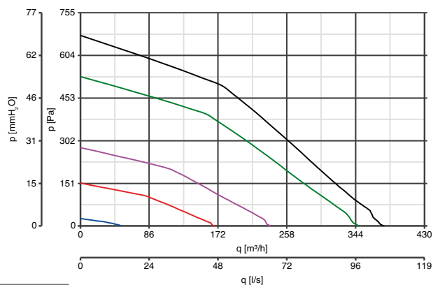
VORT PROMETEO PLUS HR 400 M CURVE PORTATA/PRESSIONE
