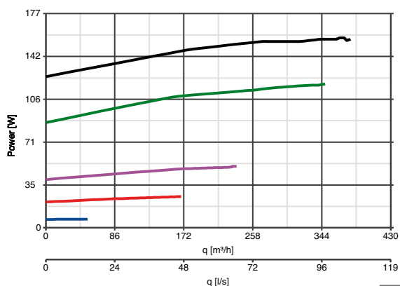
VORT PROMETEO PLUS HR 400 M CURVE ASSORBIMENTI
